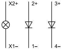
22 Switching element for Pushbutton | Keylock- and Selector switch 2 positions page 35
