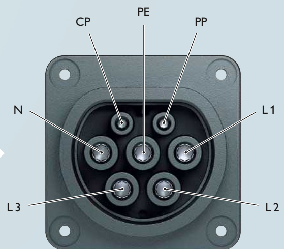
AC infrastructure socket outlet Type 2
