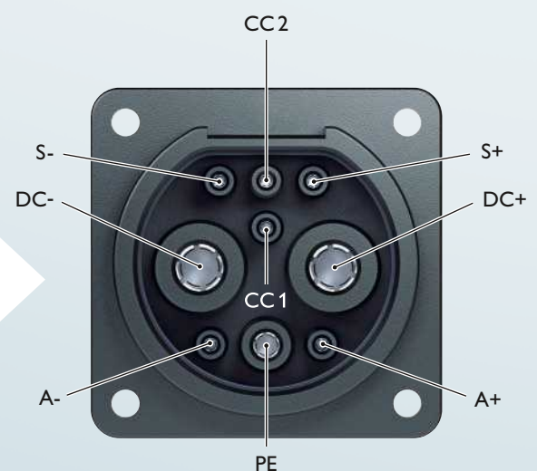
DC vehicle inlet GB/T standard
