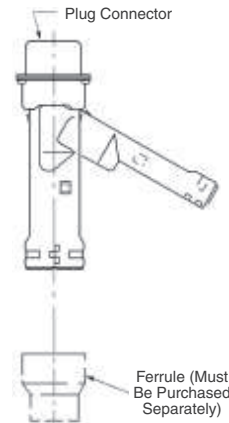
Plug Connector
