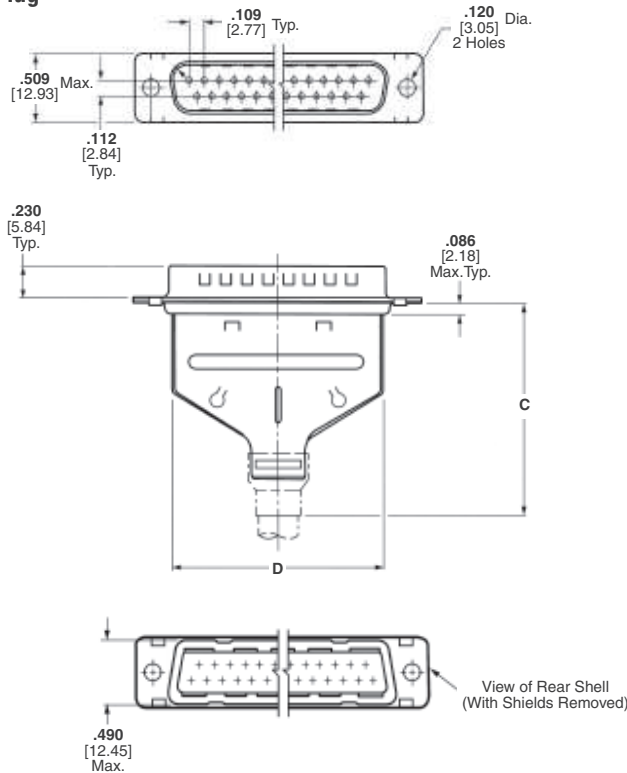
Plug Connector
