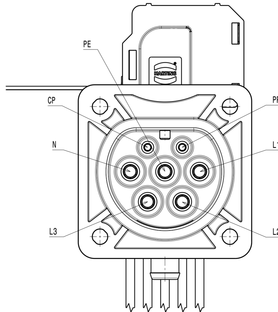
mating face acc. to IEC 62196-1:2015-06/62196-2:2017-11 M 1:1
