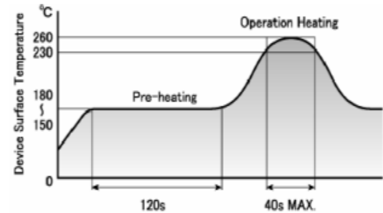
RoHS COMPLIANT SOLDER PROFILE
