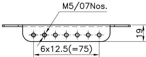
DETAIL OF MOUNTING RAIL
