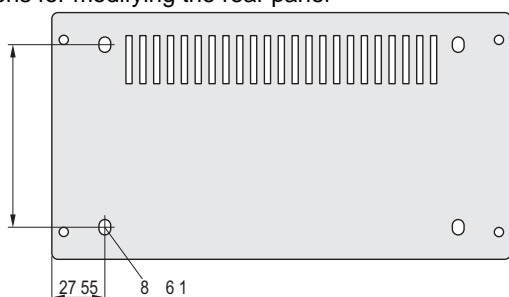
Dimensions for modifying the rear panel
