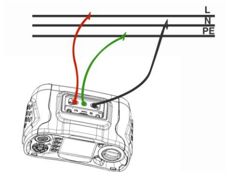
L-N Line Impedance – Test leads connection
