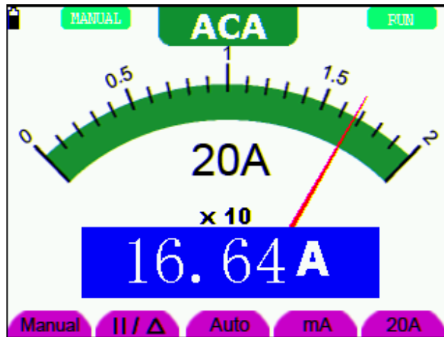
figure 27: AC Current Measurement for 20A
