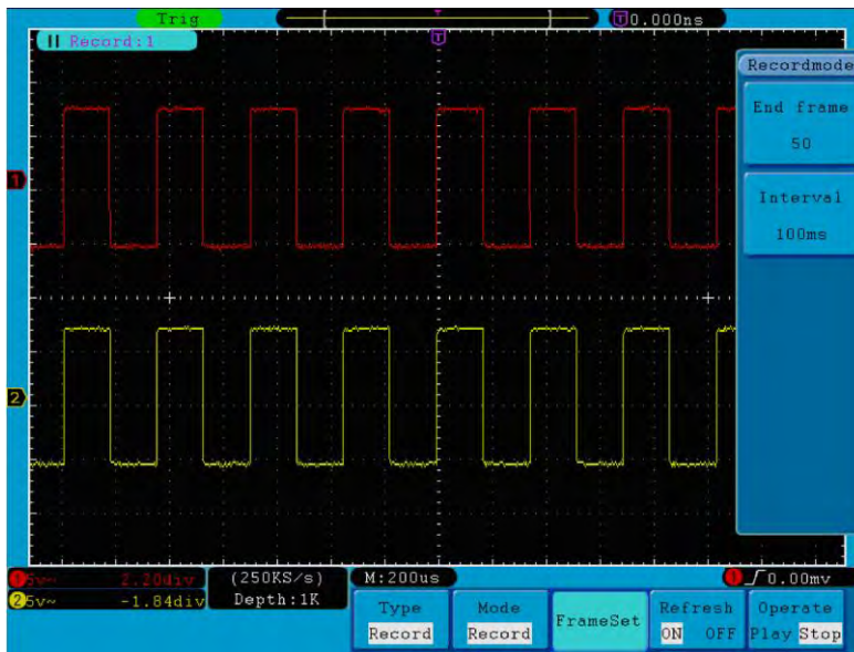
Fig. 49 Wave Record
