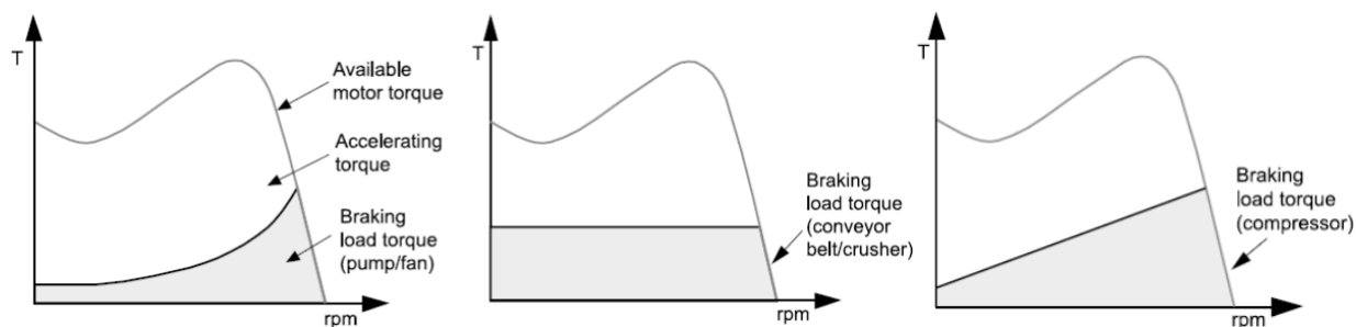
Figure 23: Diagram of the torque vs. speed for different load conditions.
