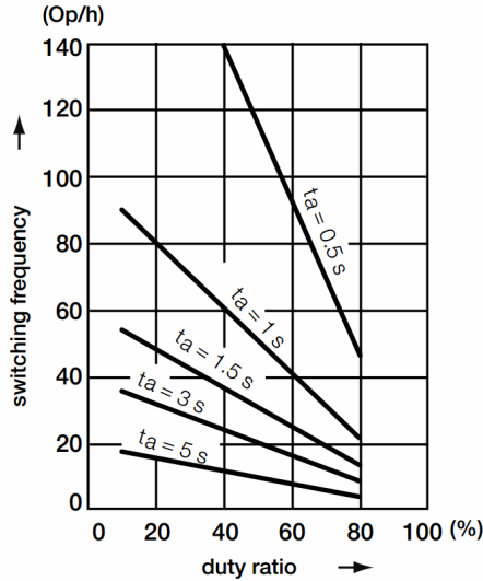
Figure 24: Diagram of the duty cycles and restarting, Example: for a motor with a duty ratio of 60 percent and a start duration of 1 second, 40 starts per hour are acceptable.
