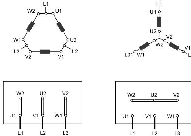
Figure 19: Voltage connection at the motor.
