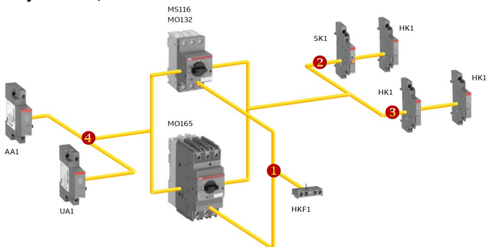
Figure 6: The maximum capacity for MS116, MO132 and MS165
