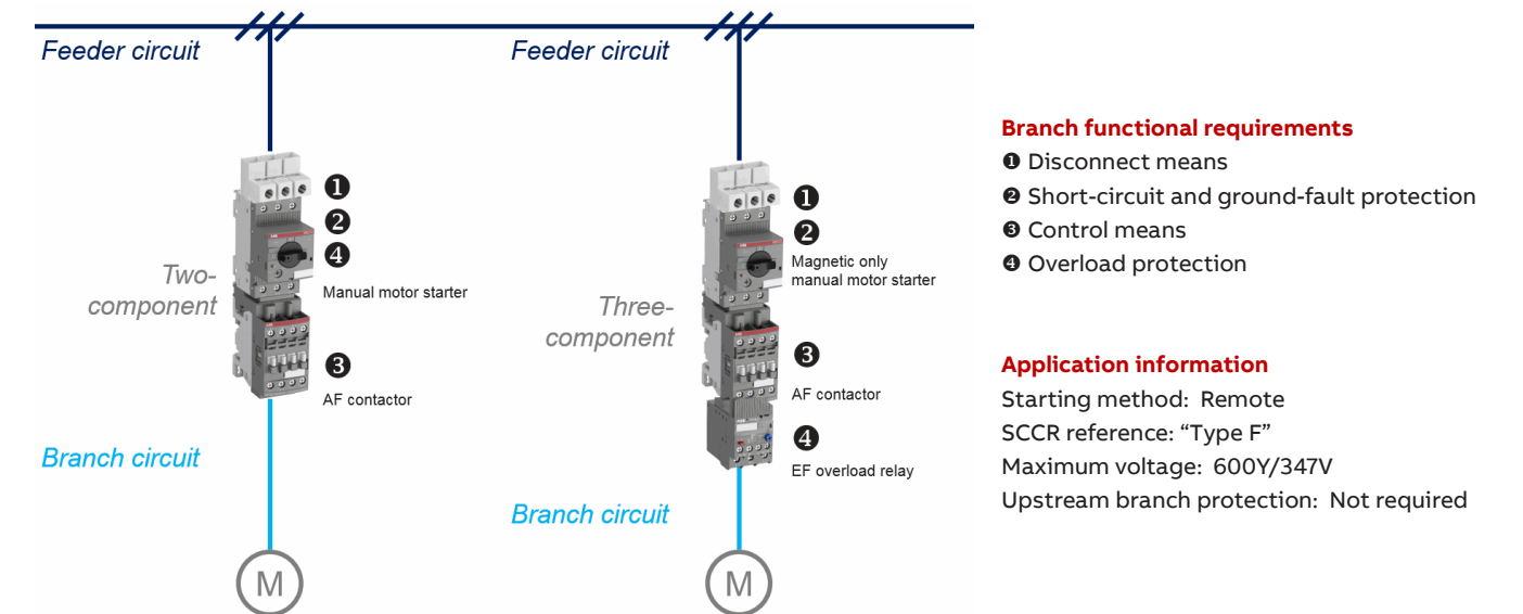
Figure 45: Combination Motor Controllers (Type F)
