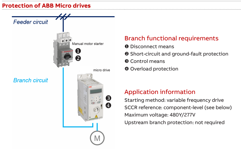
Figure 46: Protection of ABB Micro drives
