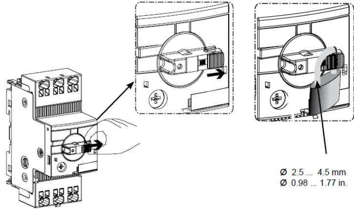
Figure 33: How to lock a manual starter by disconnecting it.
