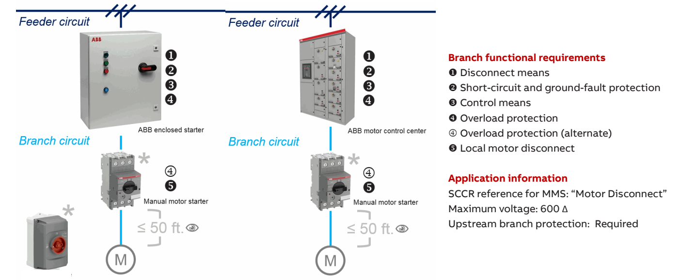
Figure 40: Manual motor starters as non-combination starters.
