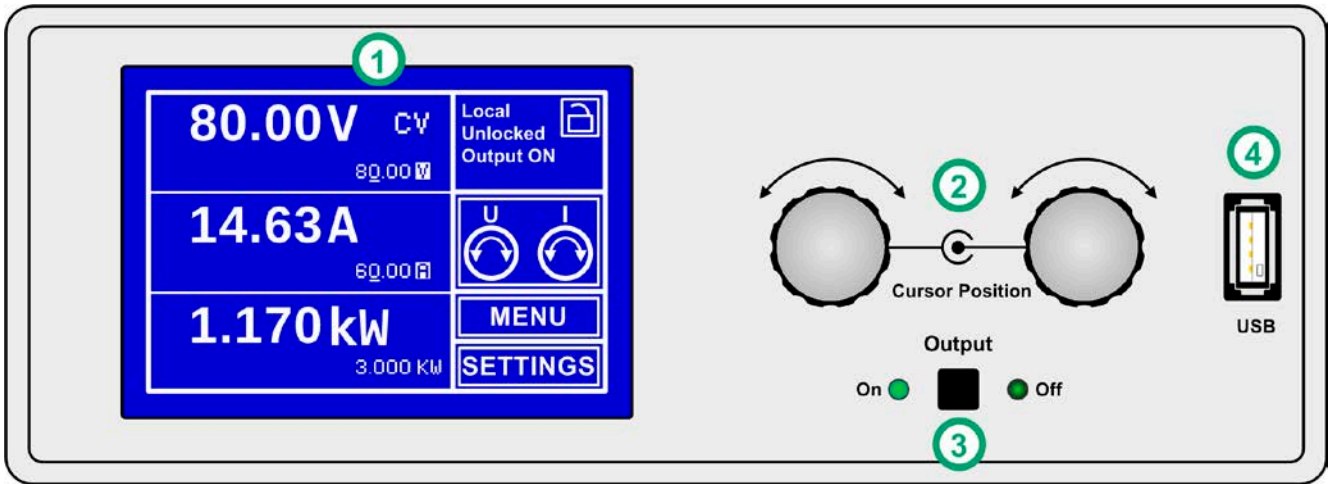
Figure 6 - Control Panel
