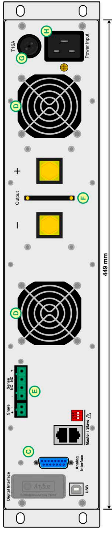
Figure 2 - Rear side
