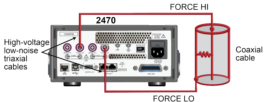
Figure 23: Rear-panel connections insulation resistance test
