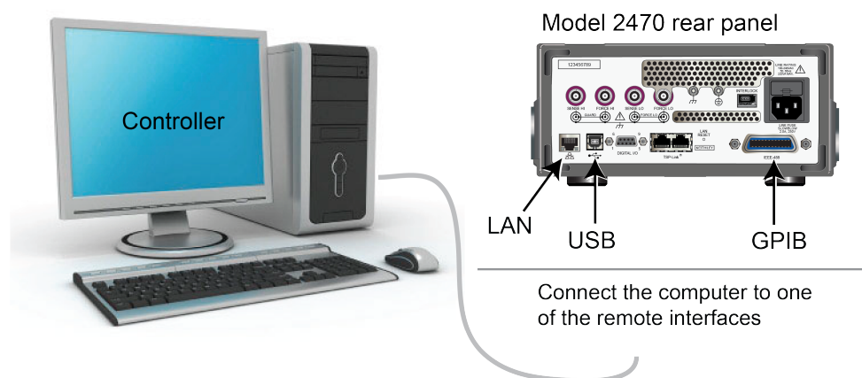
Figure 28: Model 2470 remote interface connections
