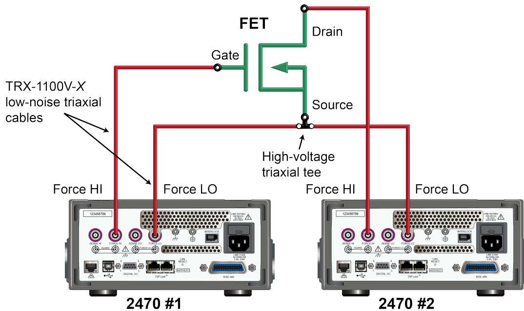
Figure 34: Two 2470s set up to test a three-terminal FET
