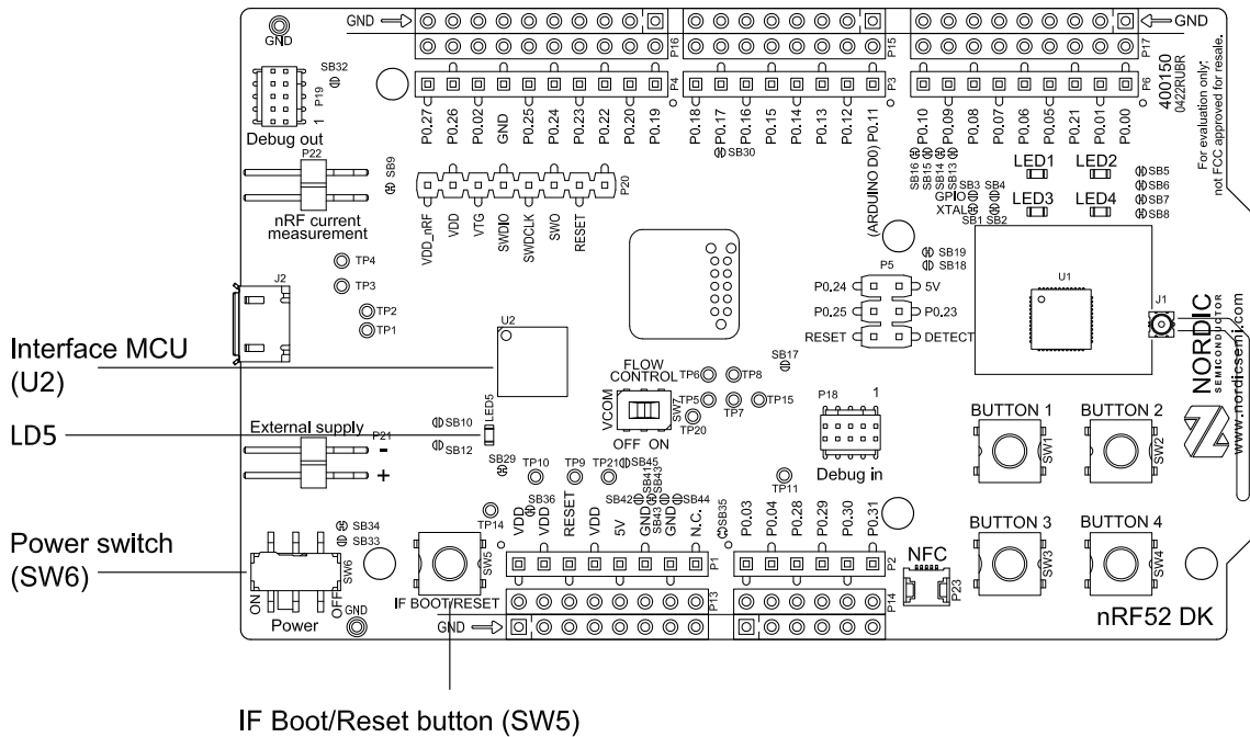
Figure 2: Interface MCU
