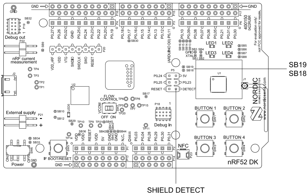
Figure 14: Enable or disable I/Os for Arduino standard
