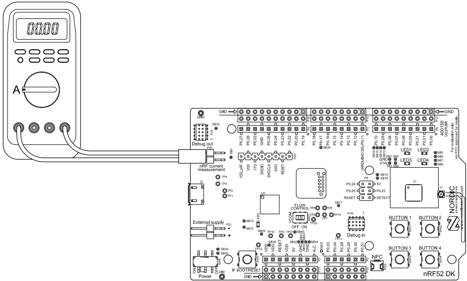
Figure 28: Current measurement with an ampere meter
