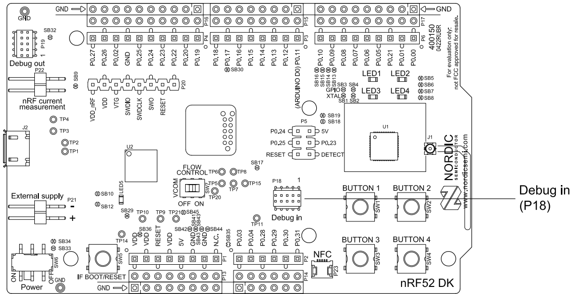
Figure 18: Debug input
