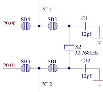
Figure 17: 32.768 kHz crystal and SB1–SB4
