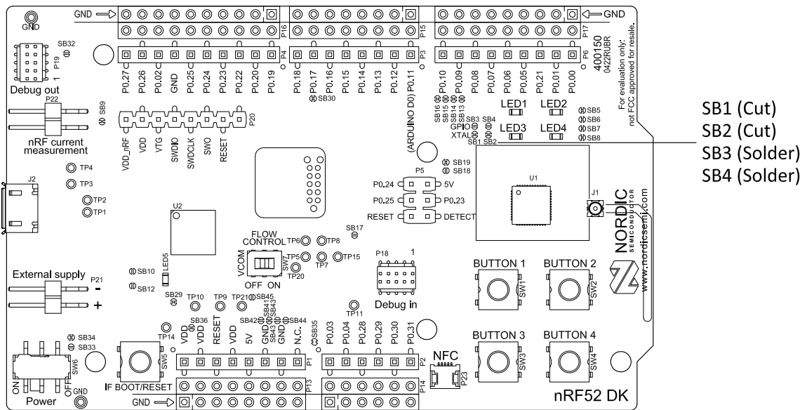
Figure 16: Configuring P0.00 and P0.01
