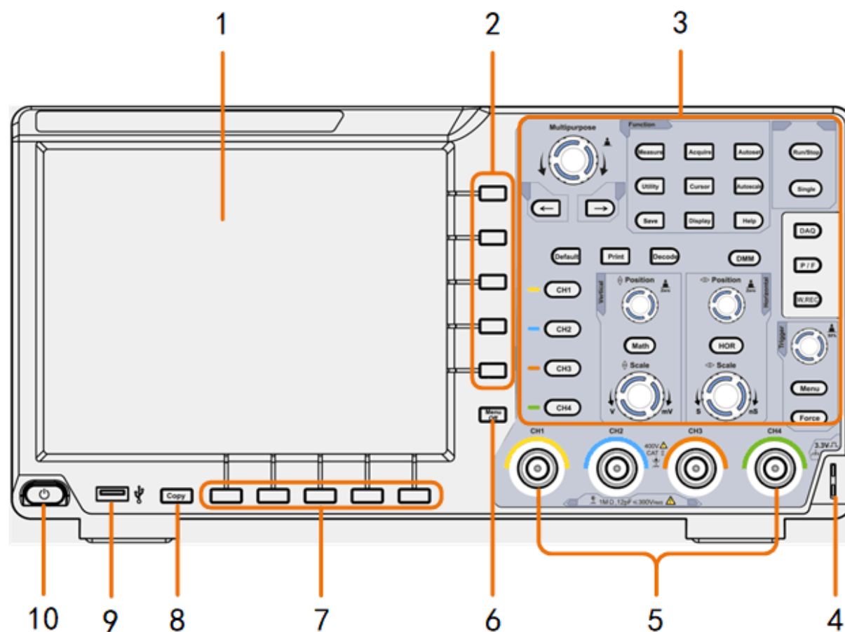
Figure 3-1 Front panel
