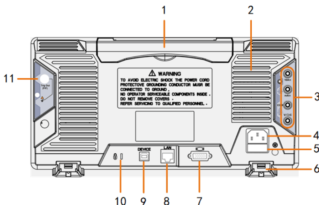
Figure 3-2 Rear Panel
