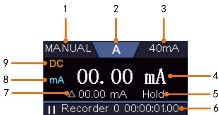
Figure 4-3 Multimeter Information Window
