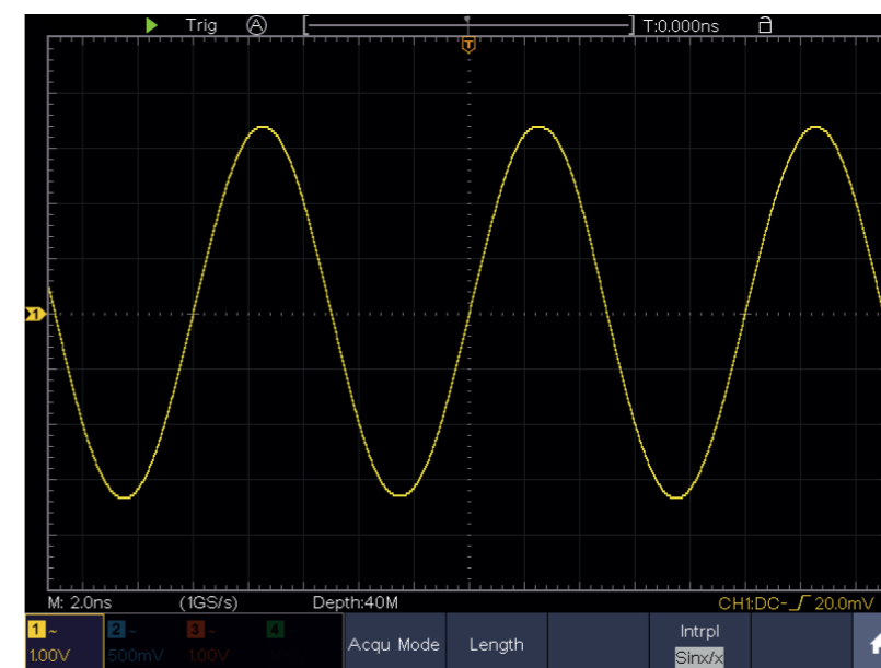
Figure 4-9 Sine( x )/ x interpolation
