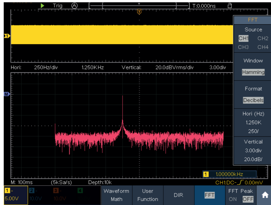
Figure 4-2 Rectangle window
