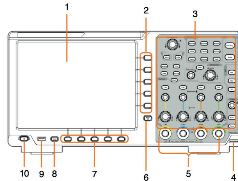
Figure 3-1 Front Panel
