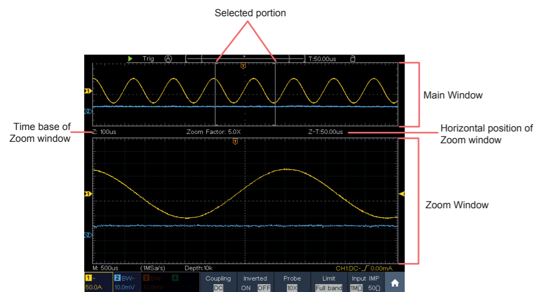
Figure 4-8 Waveform Horizontal Zooming Mode
