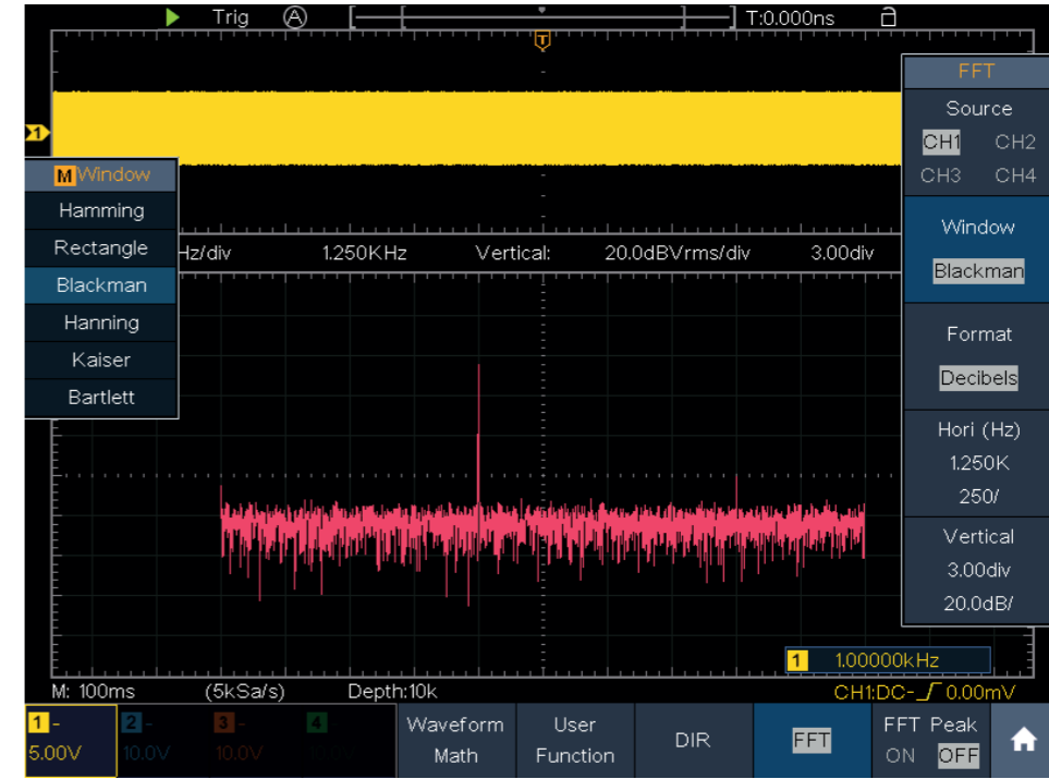
Figure 4-3 Blackman window
