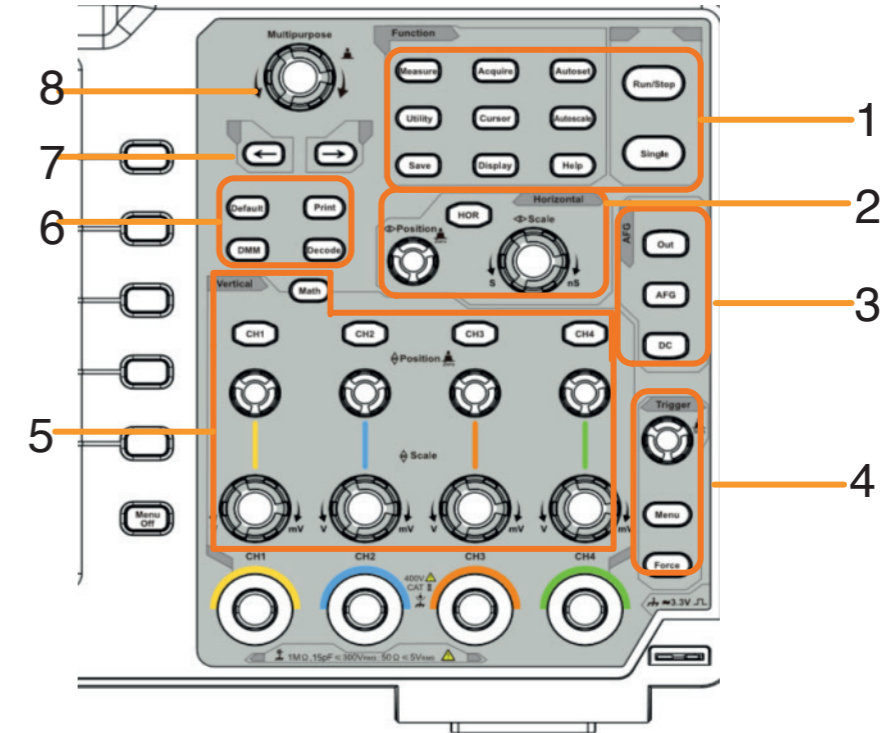
Figure 3-3 Control Area Overview
