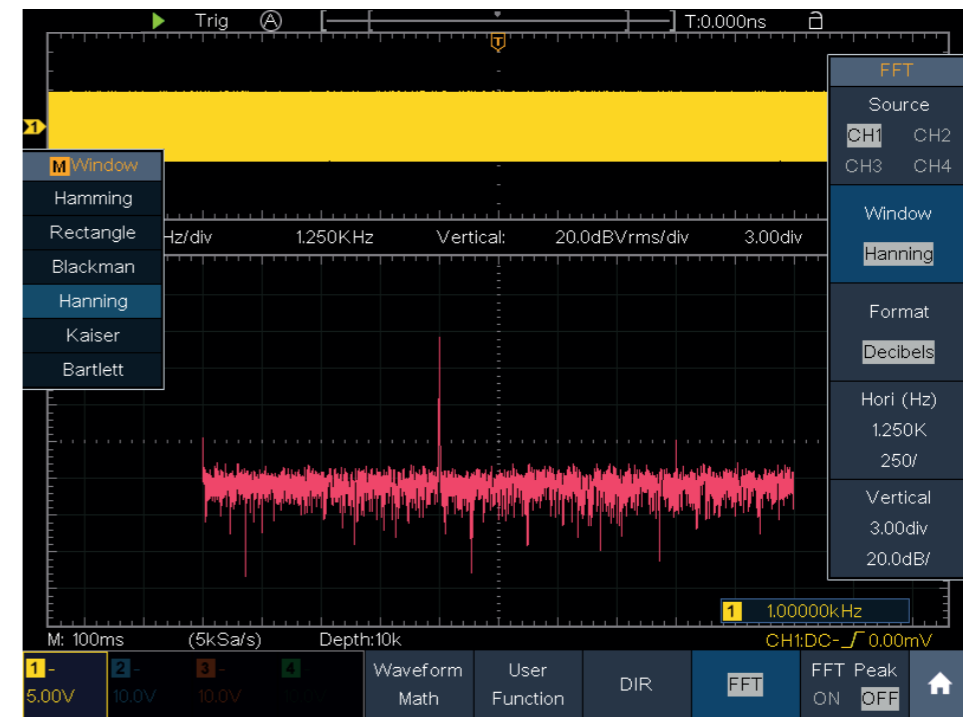
Figure 4-4 Hanning window
