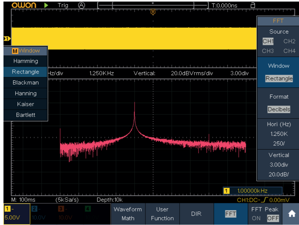
Figure 4-1 Hamming window
