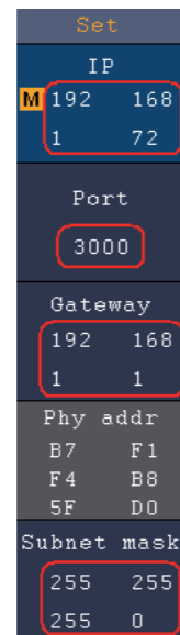
Figure 7-7 Set the network parameters of the oscilloscope
