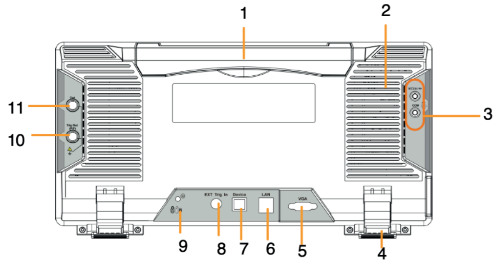
Figure 3-2 Rear Panel
