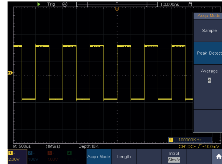
Figure 9-4 Signal with Noises
