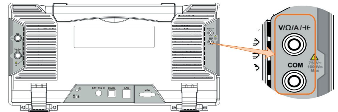
Figure 6-1 Multimeter Input Terminals
