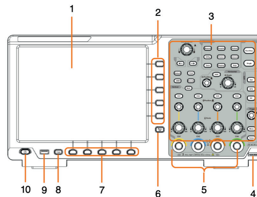
Figure 3-1 Front Panel
