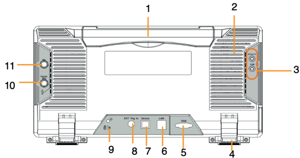
Figure 3-2 Rear Panel
