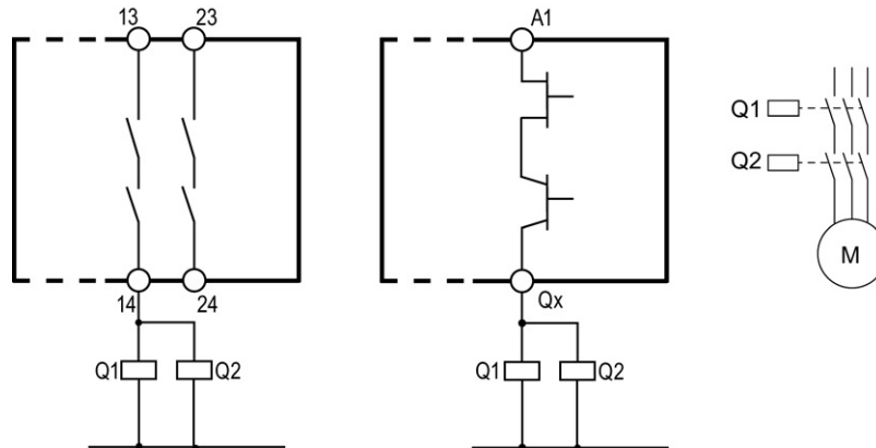
Figure 4-6 PL e/Cat. 4 in accordance with ISO 13849-1 or SILCL 3 in accordance with IEC 62061 With units that have solid-state outputs, this wiring is only possible from E02/V1.1.0.
