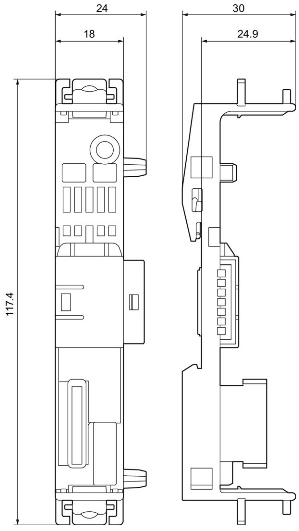
Figure 14-10 Device connector for 3SK1 safety relays, width: 17.5 mm
