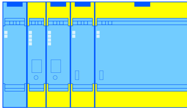
Typical 3SK1 Advanced system configuration
