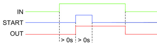
Figure 4-3 Start function "Manual start"
