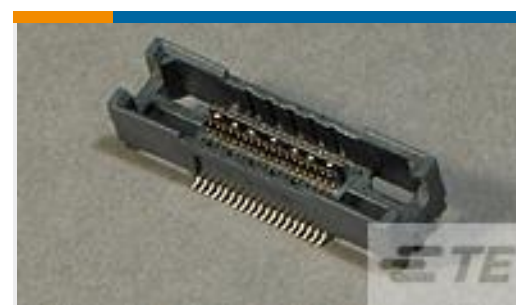
TE Part #2-5767004-2 MICTOR RECEPT ASSY, 38 POS.
