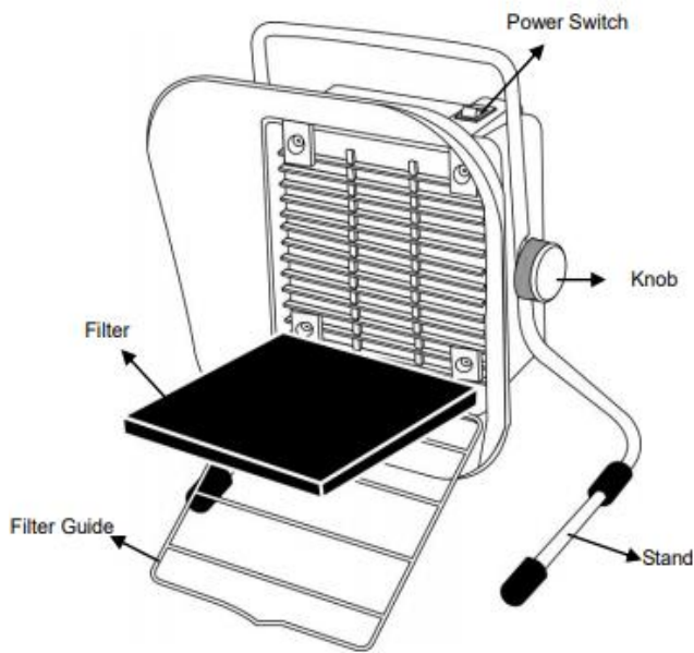
Activated-Carbon Filter (2 pieces included)
