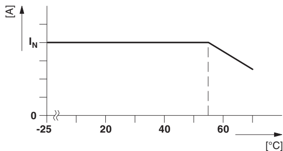
Figure 13 Temperature-dependent derating
