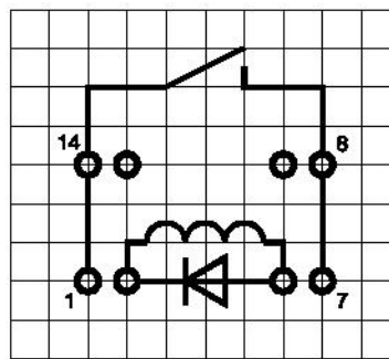
Layout 11D/ Pitch 2,54 / Top View
