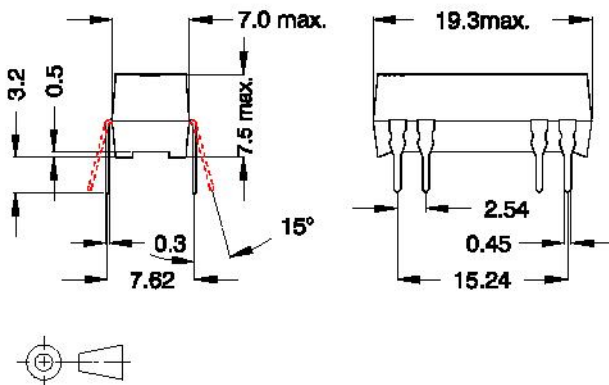
Dimensions (tolerance \pm 0,1\text{mm} )
