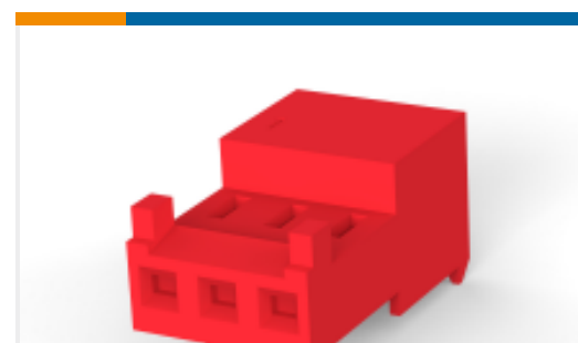
TE Part #4-643813-0 Nylon Tin Plated Receptacle: 2.54mm, With Mating Alignment, MTA 100
