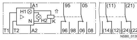
3RN10 11, 2 COs
