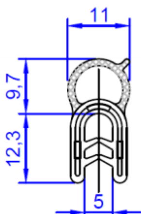
Clamping Range 1-3mm Black EPDM 60 \pm 5 Shore, Including Looped Wire Carrier & Hollow Sponge Sealing Section
