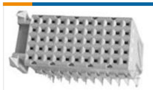
TE Part #5100161-9 Z-PACK 2mm HM/C RAF 55P
