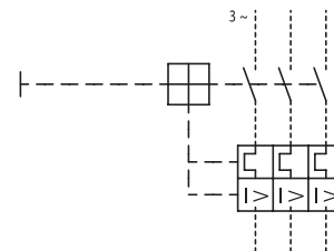
Three-phase operation
