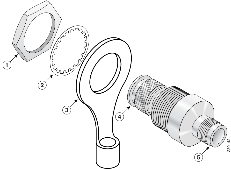
Figure 1 Lightning Arrestor Details
