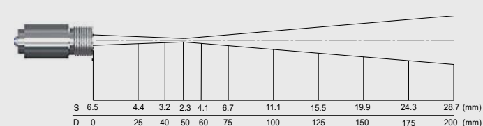
CF optics, D:S = 22:1 (far field = 6:1)
