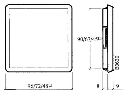
Cut-out cover
