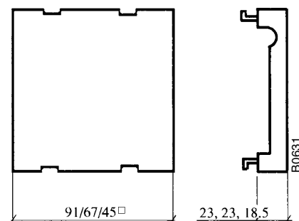
Protection cover
