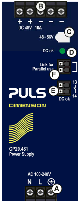
Fig. 11-1 Front side
