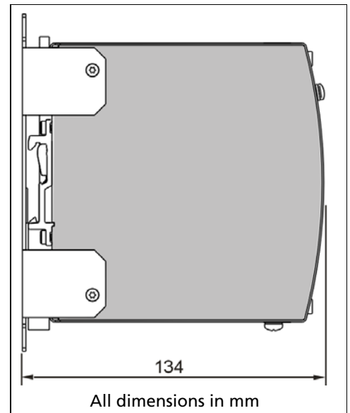
Fig. 22-6 Wall/panel mounting, side view (Picture shows the CP20.241)
