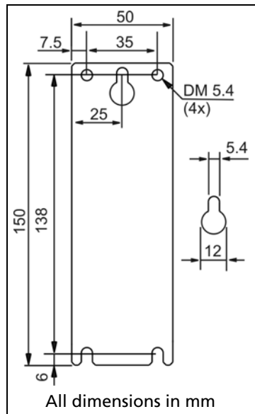
Fig. 22-5 Hole pattern for wall mounting
