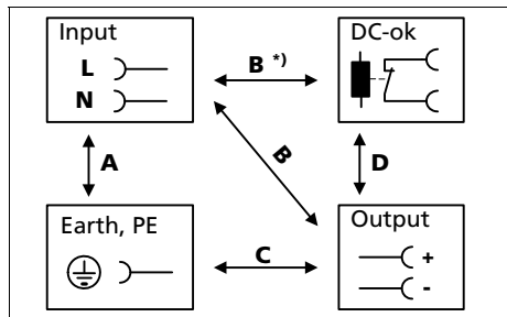
Fig. 18-1 Dielectric strength
