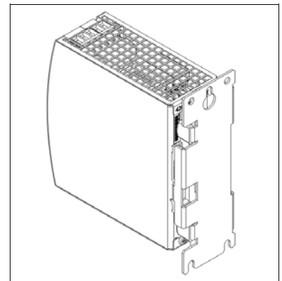
Fig. 22-3 Isometric view (Picture shows the CP20.241)
