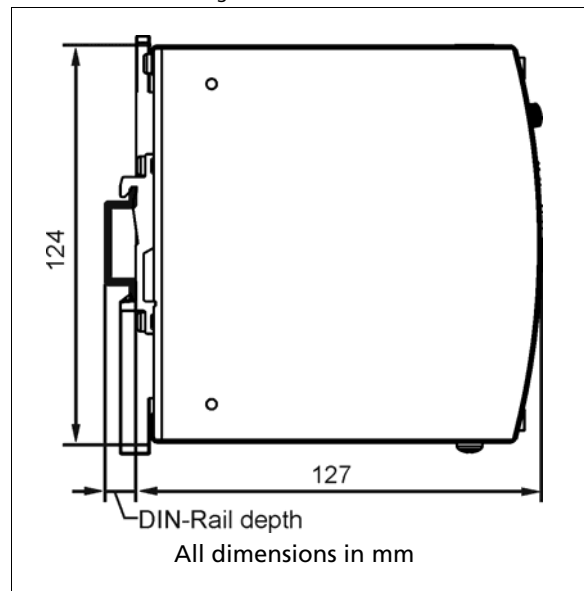
Fig. 21-2 Side view
