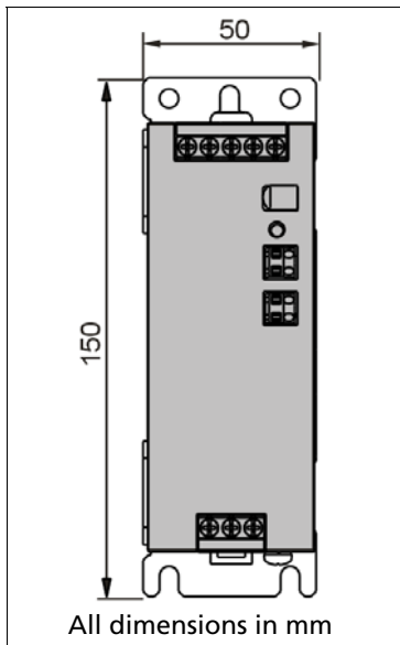
Fig. 22-4 Wall/panel mounting, front view (Picture shows the CP20.241)
