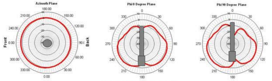
Figure 4-3 Outdoor Omnidirectional Antenna Radiation Patterns (2 of 2)
