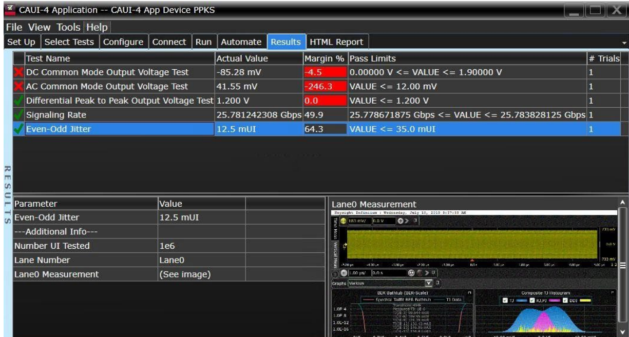
Figure 5. The D9010CAUC CAUI-4 compliance test application software results screen shows a summary of the tests performed, pass/fail status, and margin. Clicking on a specific test also shows the test specification and a measurement waveform, if appropriate.
