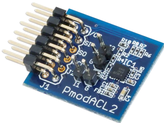
The PmodACL2.
