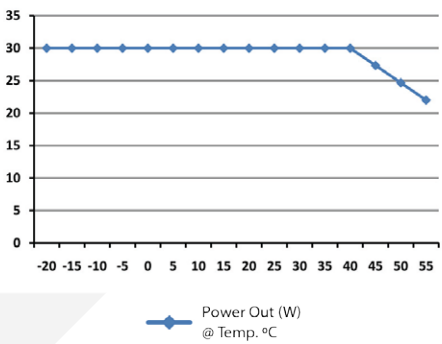
PD-9001GR Performance
