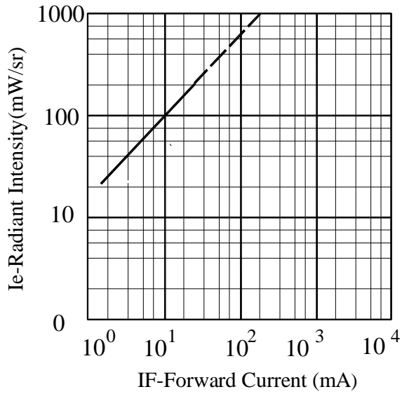
Radiant Intensity vs. Forward Current
