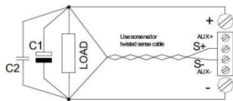
Remote Sensing (fig.6)
