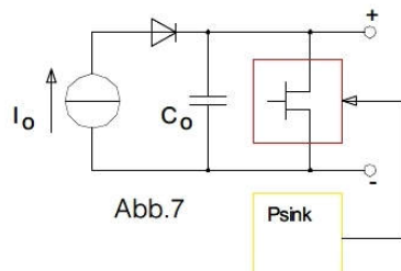
Power sink equipped power supply
