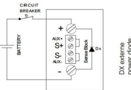
Battery Charger Mode (fig.7)
