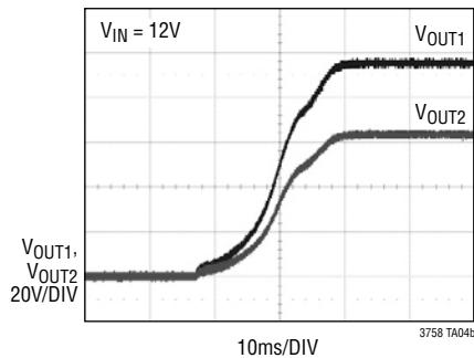
Start-Up Waveforms
