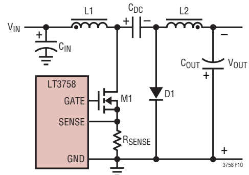
Figure 10. A Simplified Inverting Converter
