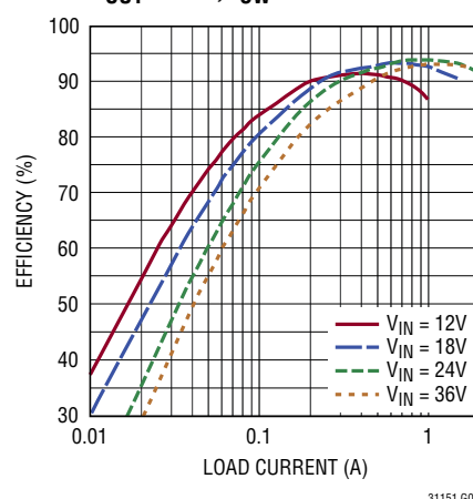
PWM Mode Efficiency, V_{OUT} = 24V , f_{SW} = 1\text{MHz}
