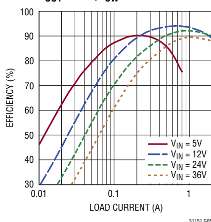
PWM Mode Efficiency, V_{OUT} = 12V , f_{SW} = 1\text{MHz}
