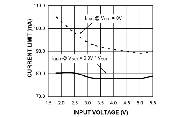
FIGURE 2-4: MIC2090 Current-Limit vs. Input Voltage.
