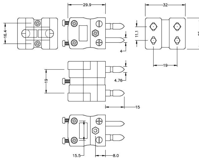
Standard Duplex in-line Plug (dimensions in mm)
