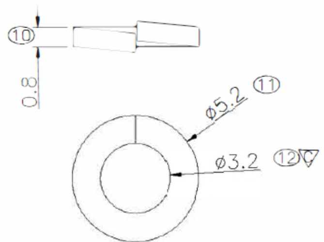
Spring gasket
