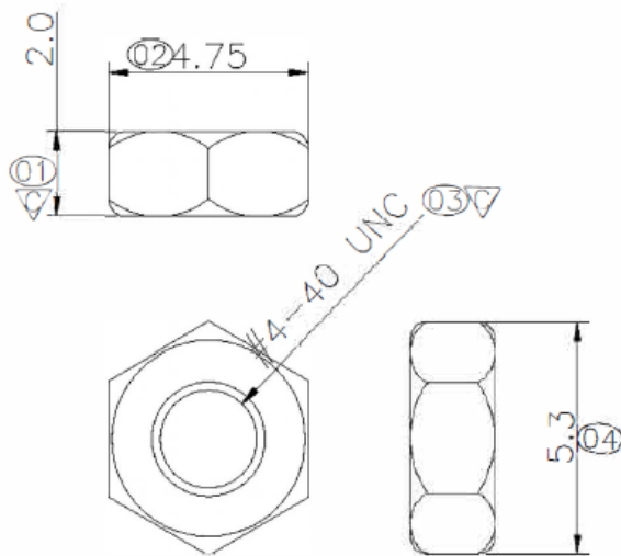
Screw cap
