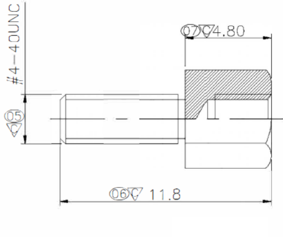
Screw
