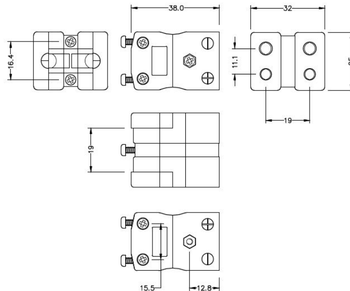
Standard Duplex in-line Socket (dimensions in mm)
