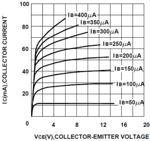
STATIC CHARACTERISTIC
