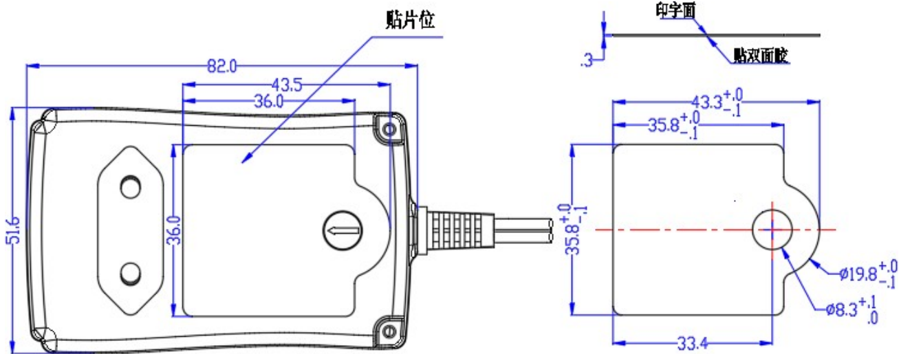
贴片2TP-3R15U
