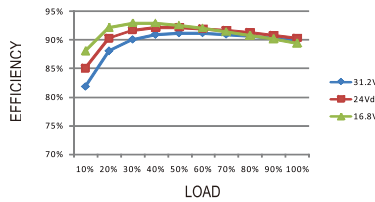
RSD-300C-5
