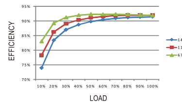
RSD-300D-24
