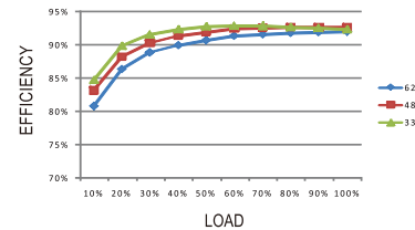
RSD-300D-24
