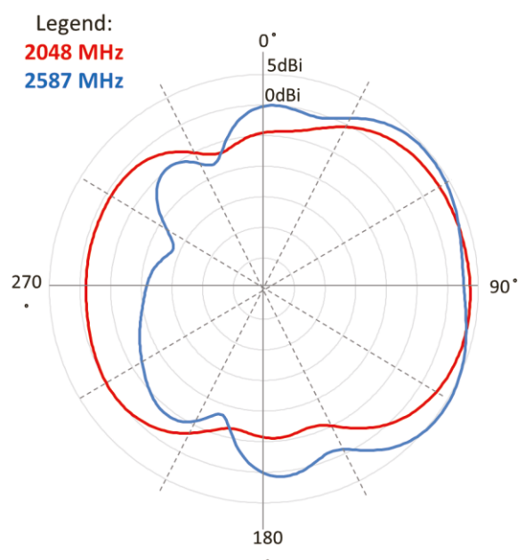
Elevation 2(YZ)
