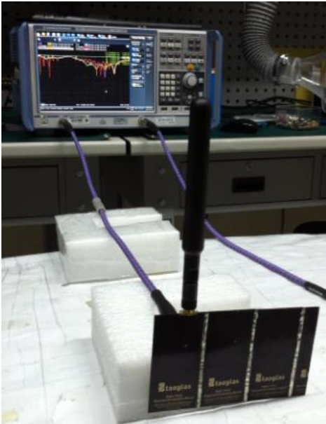
Antenna straight
