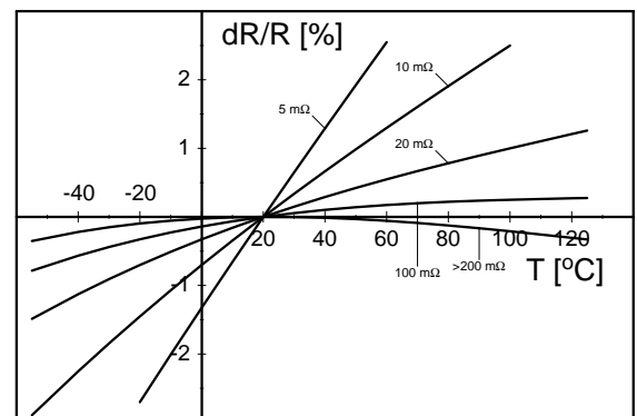
Change of the R(T)-curve to the TCR of copper terminals for very low ohmic 2-terminal-resistors
