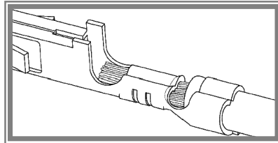
Figure 9-13 CONDUCTOR BRUSH TOO LONG
