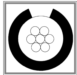
Figure 9-19 ACCEPTABLE INSULATION CRIMP
