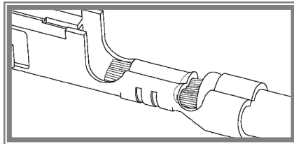
Figure 9-5 OPTIMAL CRIMP
