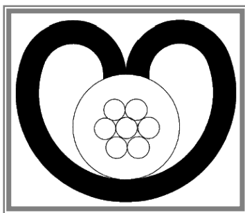
Figure 9-22 MARGINAL INSULATION CRIMP
