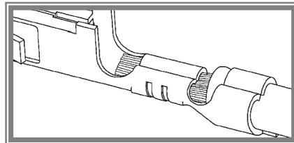
Figure 9-8 NO BELL MOUTH, EXCESSIVE CUT-OFF TAB
