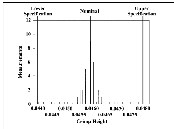
Figure 9-25 OPTIMAL CRIMP HEIGHT CHART
